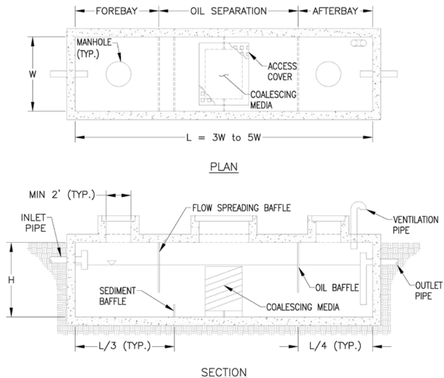
Figure 15-2 Enhanced Gravity Oil Water Separator
