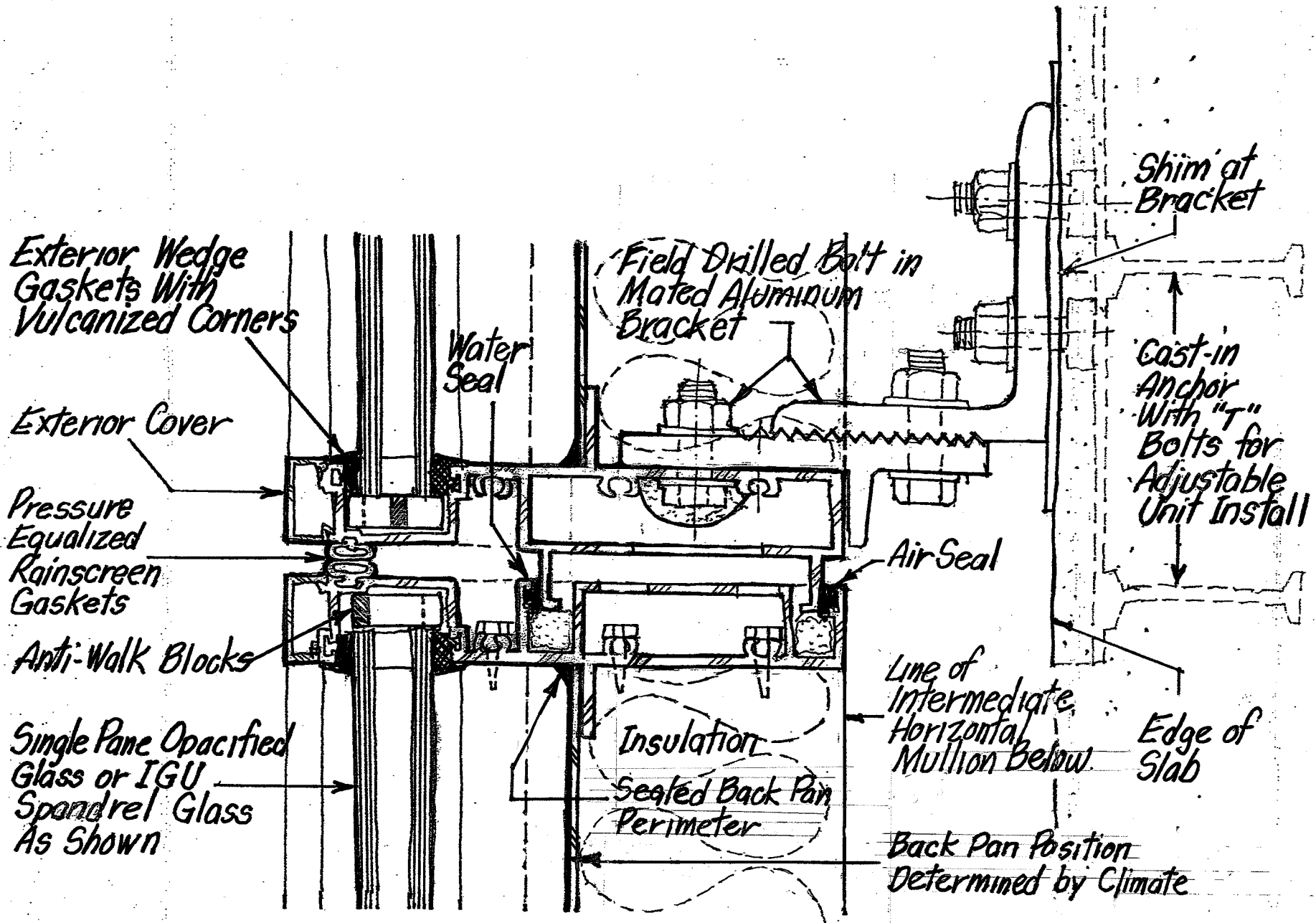
FIGURE U-7 JAMB AT SPANDREL GLASS AND ANCHORAGE TO SLAB UNITIZED CURTAIN WALL
