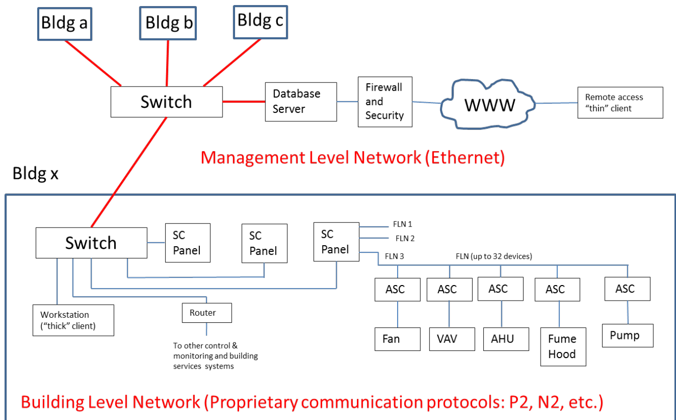
Figure 7.2.1.2 The NIH Bethesda Campus Building Automation System Network Layout
