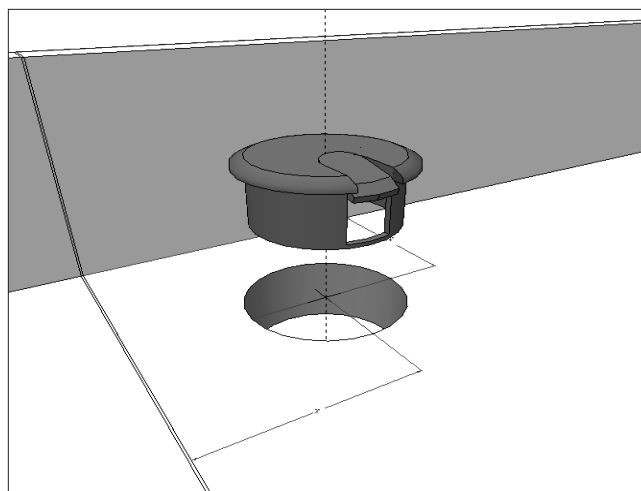
Figure 4.5.2.2 Grommet Detail
