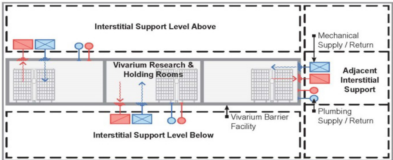
Figure 2.3.2.8 Utility distribution strategies
