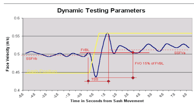
Figure E.3.A Dynamic Testing Parameters
