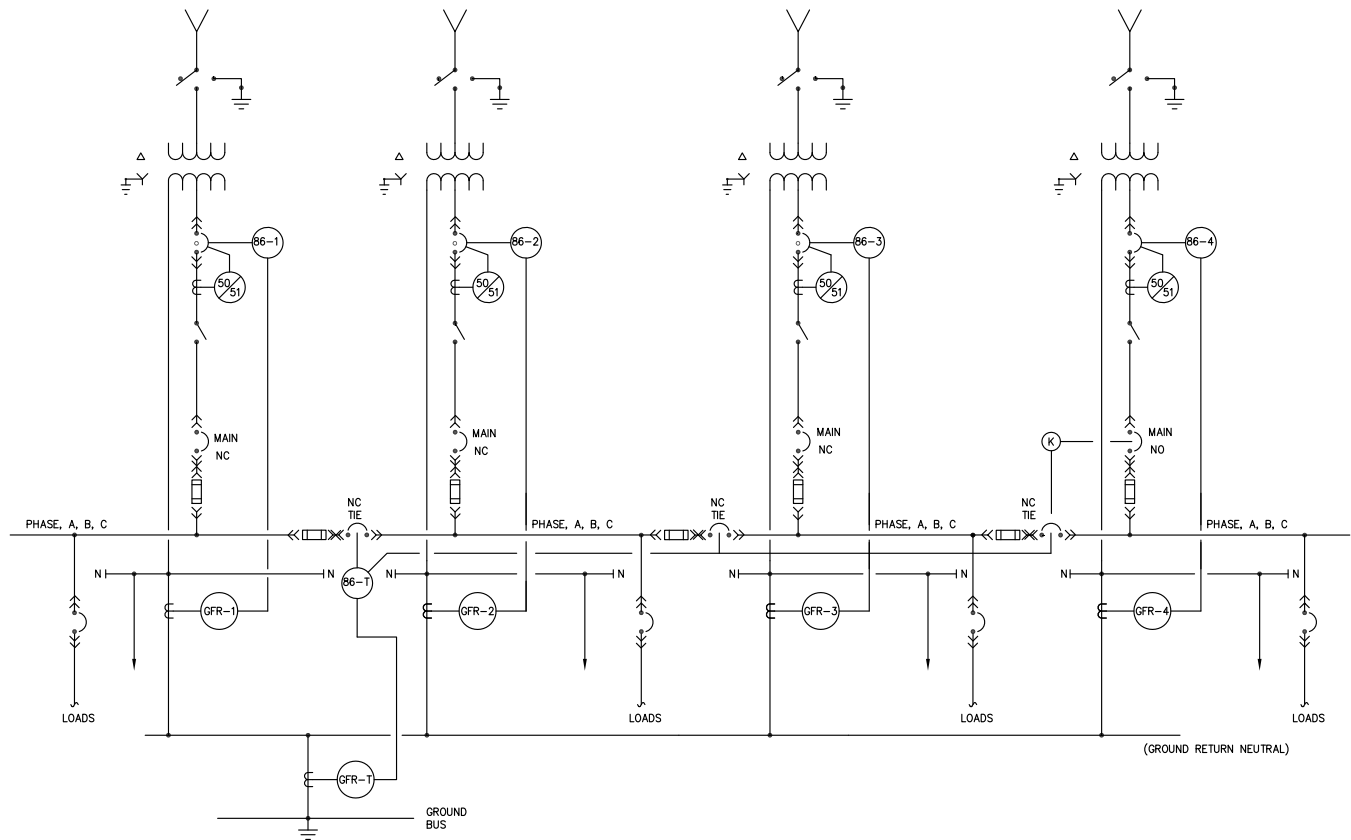
Figure 10.2.1(B) Typical building service (four transformers) – normal power (Fourth transformer is for emergency power)
