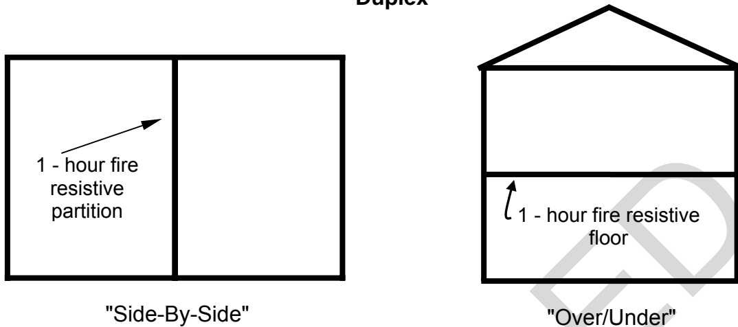
Figure 6-6 Duplex
