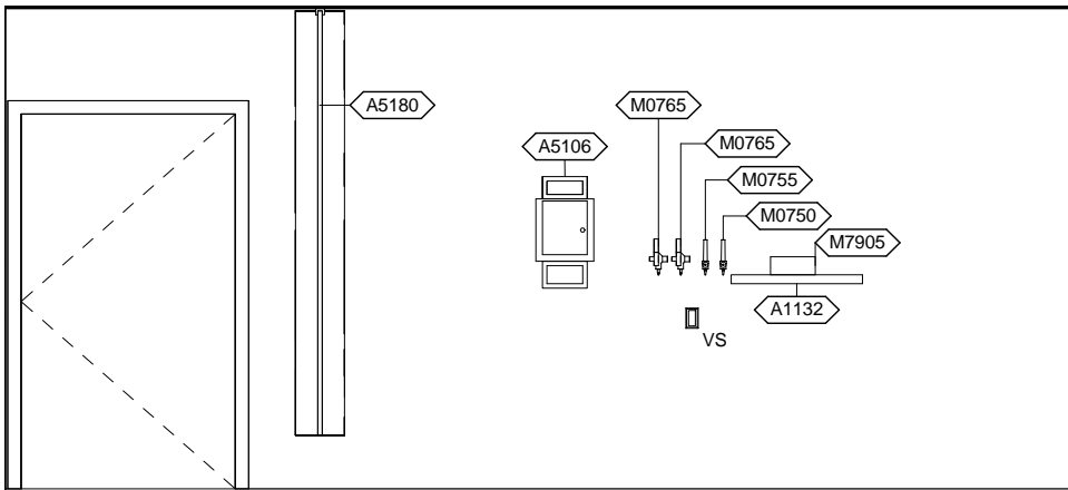
TRPE1 - SOUTH ELEVATION
