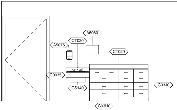
DNTS1 - SOUTH ELEVATION
