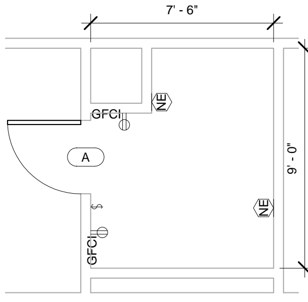
TLTS1 - FLOOR PLAN
