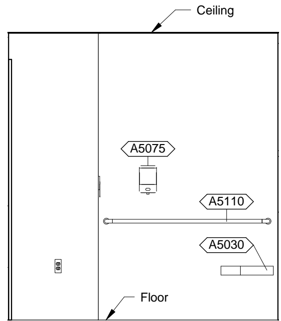
TLTS1 - PLAN NORTH
