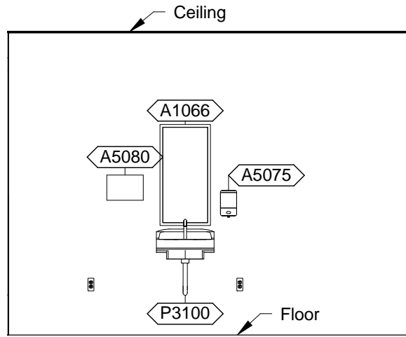
OPTM1 - PLAN EAST
