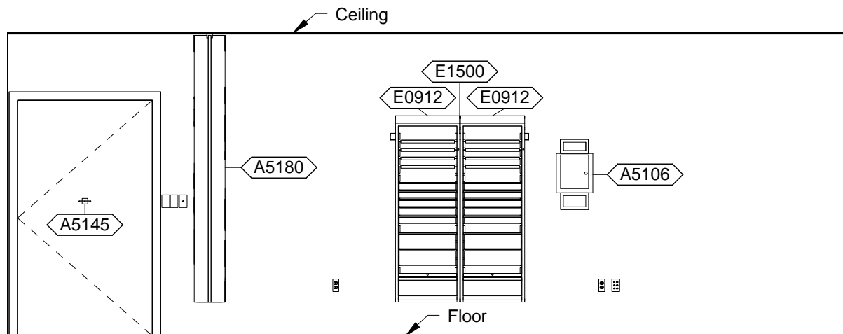
OPTM1 - PLAN SOUTH
