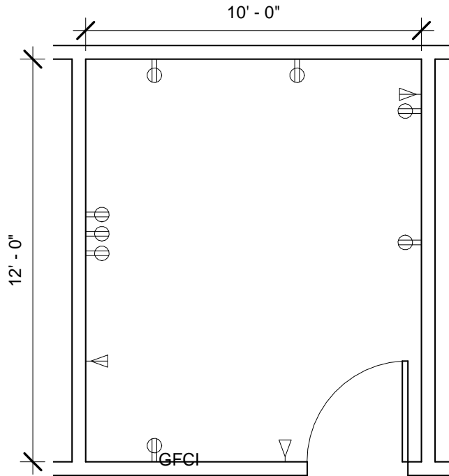
EYVS1 - FLOOR PLAN
