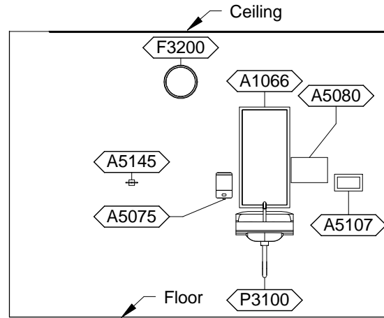
DNXC1 - PLAN SOUTH
