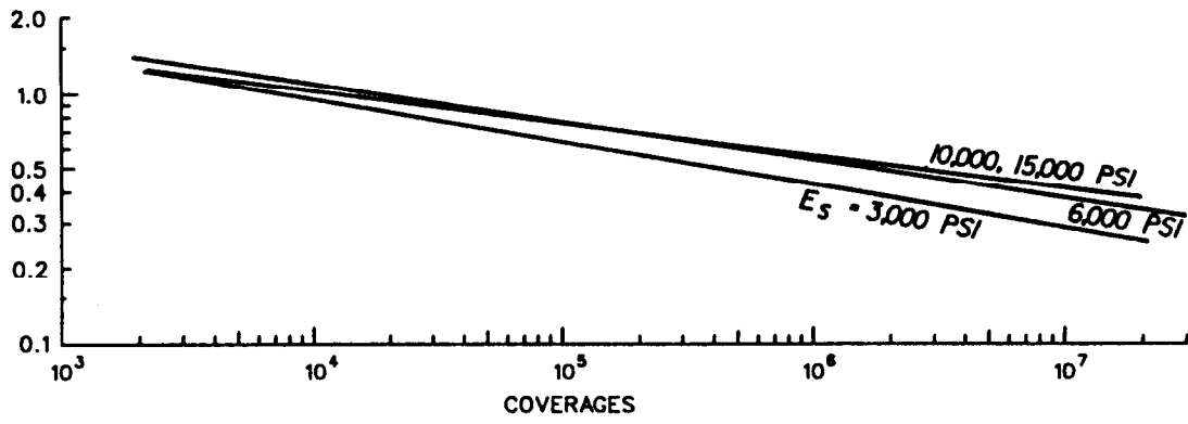
Figure 5-1. Subgrade Strain Criteria for Roads and Streets.
