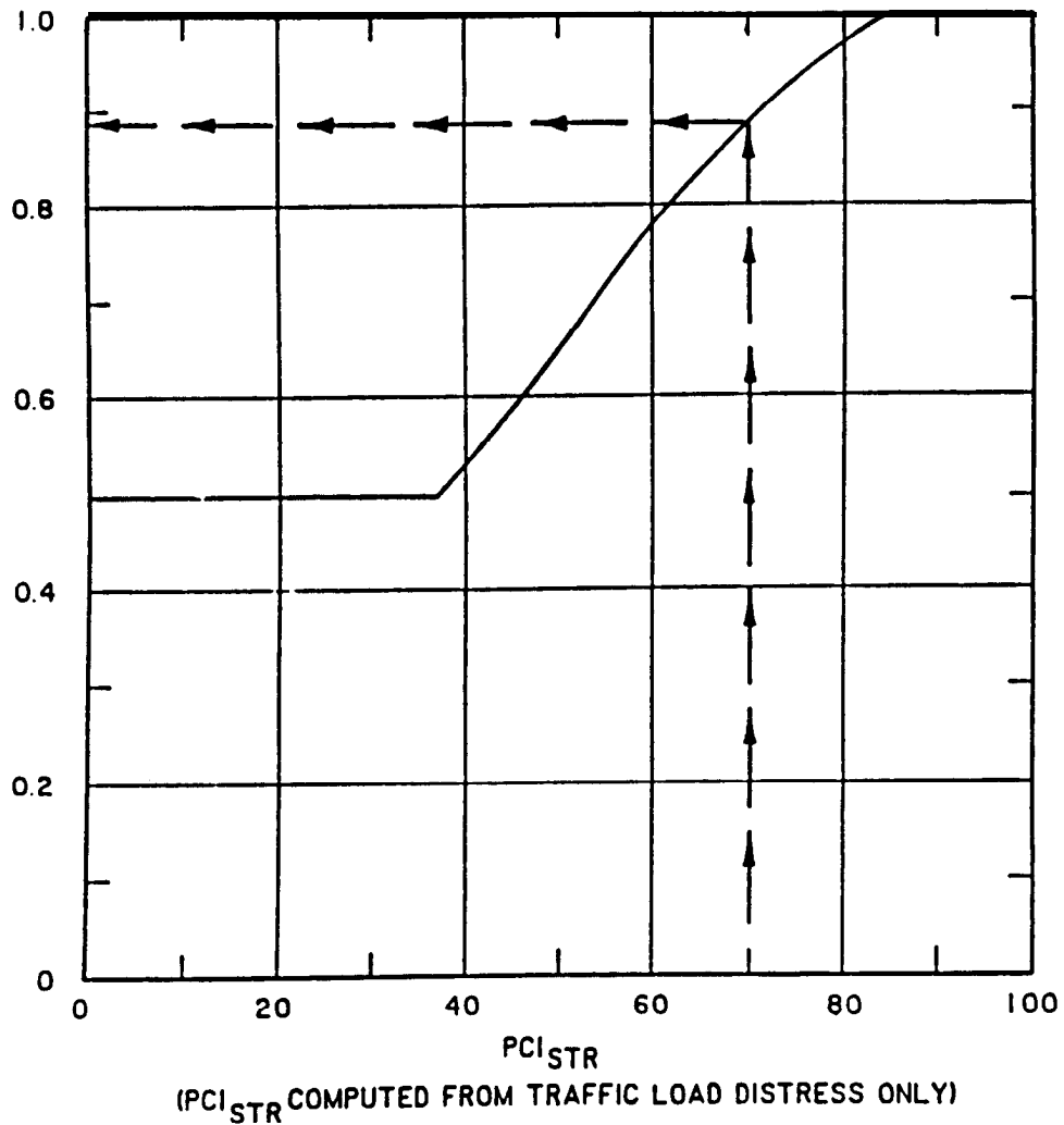
Figure 8-2. Chart for Determining C_s for Flexible Overlays.
