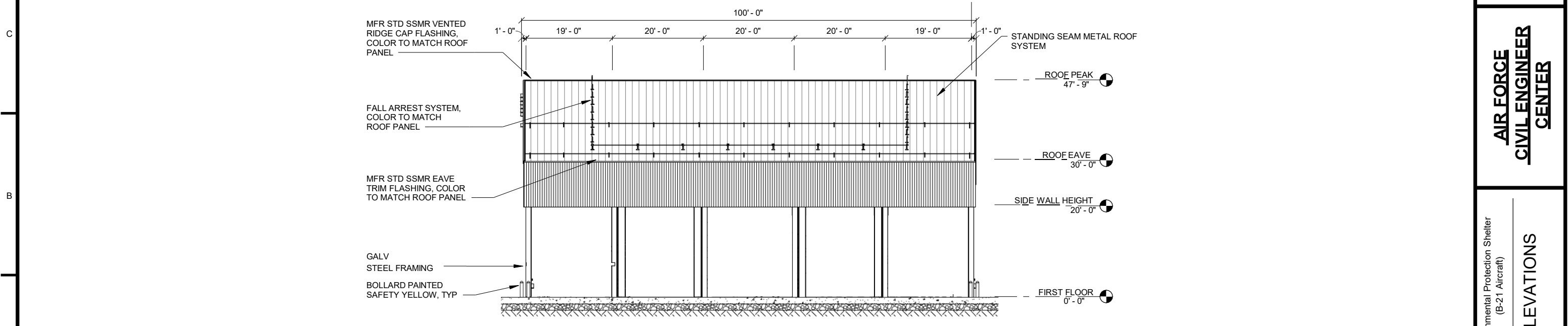
2 EXTERIOR ELEVATION - EPS SIDES
