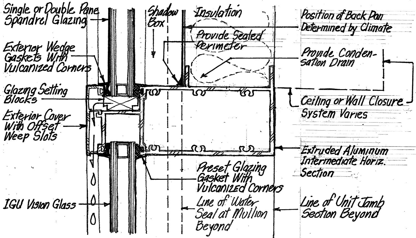
FIGURE U-6 INTERMEDIATE HORIZONTAL UNITIZED CURTAIN WALL
