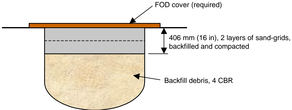
Figure 2-2. Sand Grid Repair
