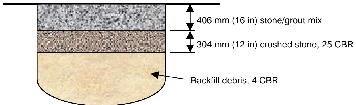
Figure 2-3. Stone and Grout Repair
