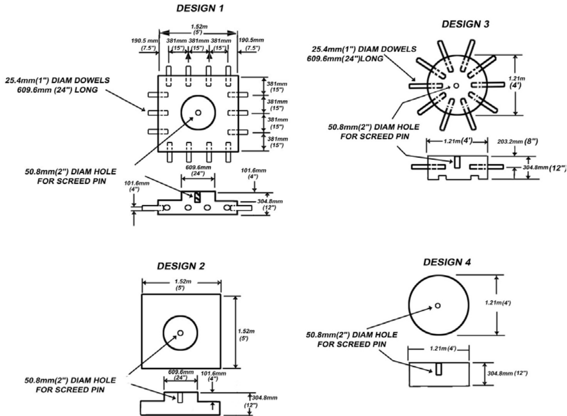
Figure 2-5. Pedestal Designs
