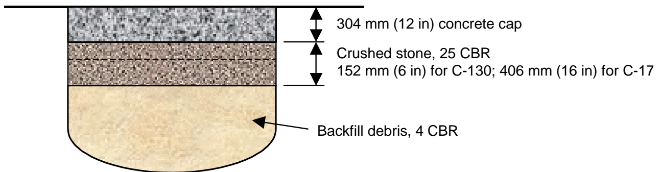
Figure 2-4. Concrete Cap Repair
