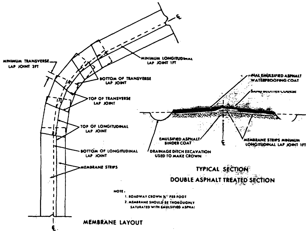
Figure 3-4. Polypropylene membrane layout for curved sections.
