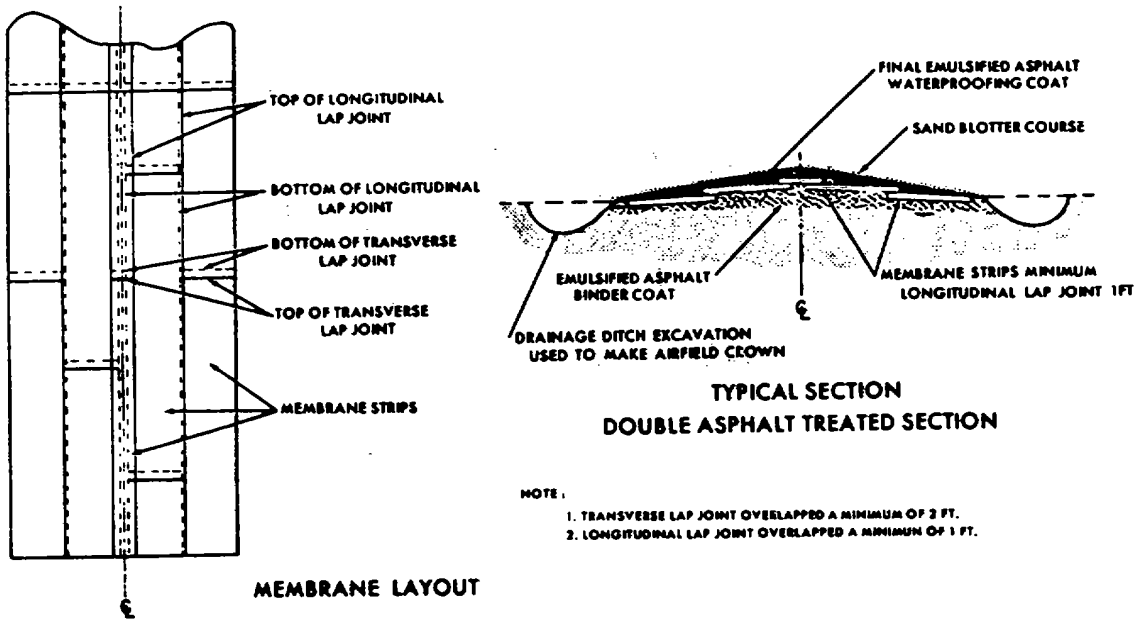
Figure 3-3. Polypropylene membrane layout for tangential sections.
