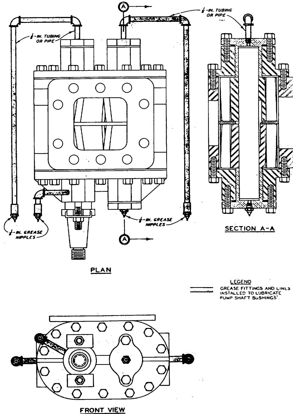
Figure 5-1. Typical pump modifications for conventional asphalt distributor.
