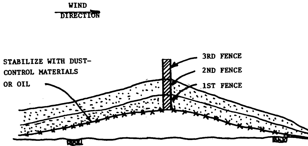
Figure B-3. Cross section of dune showing initial and subsequent fences.
