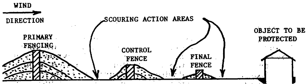
Figure B-4. Three fences installed to control dune formation
