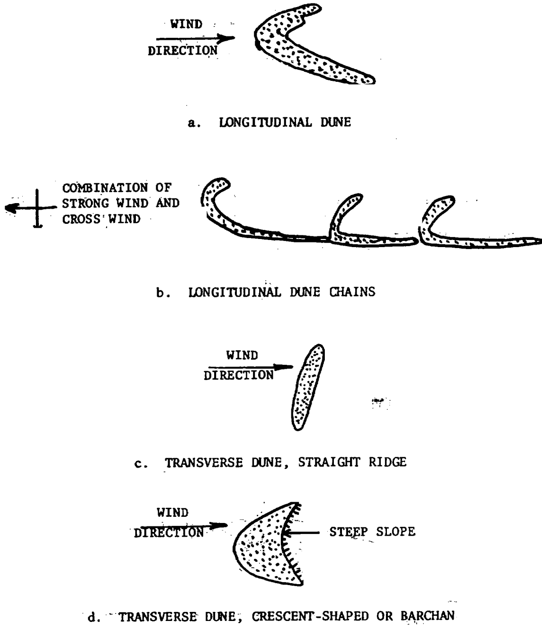
Figure B-2. Types of moving sand dunes
