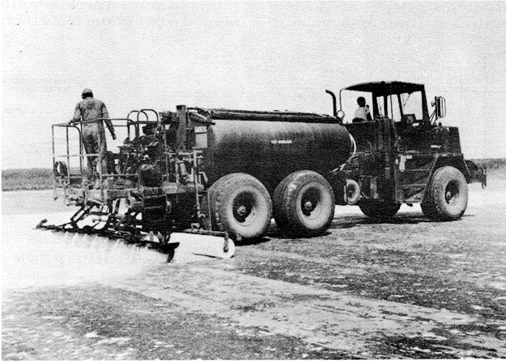
Figure 3-1. Special distributor for the three-step process of applying the DCA 1295.
