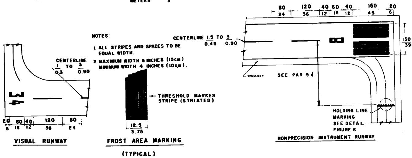
Figure 2-3. Visual and nonprecision marking.
