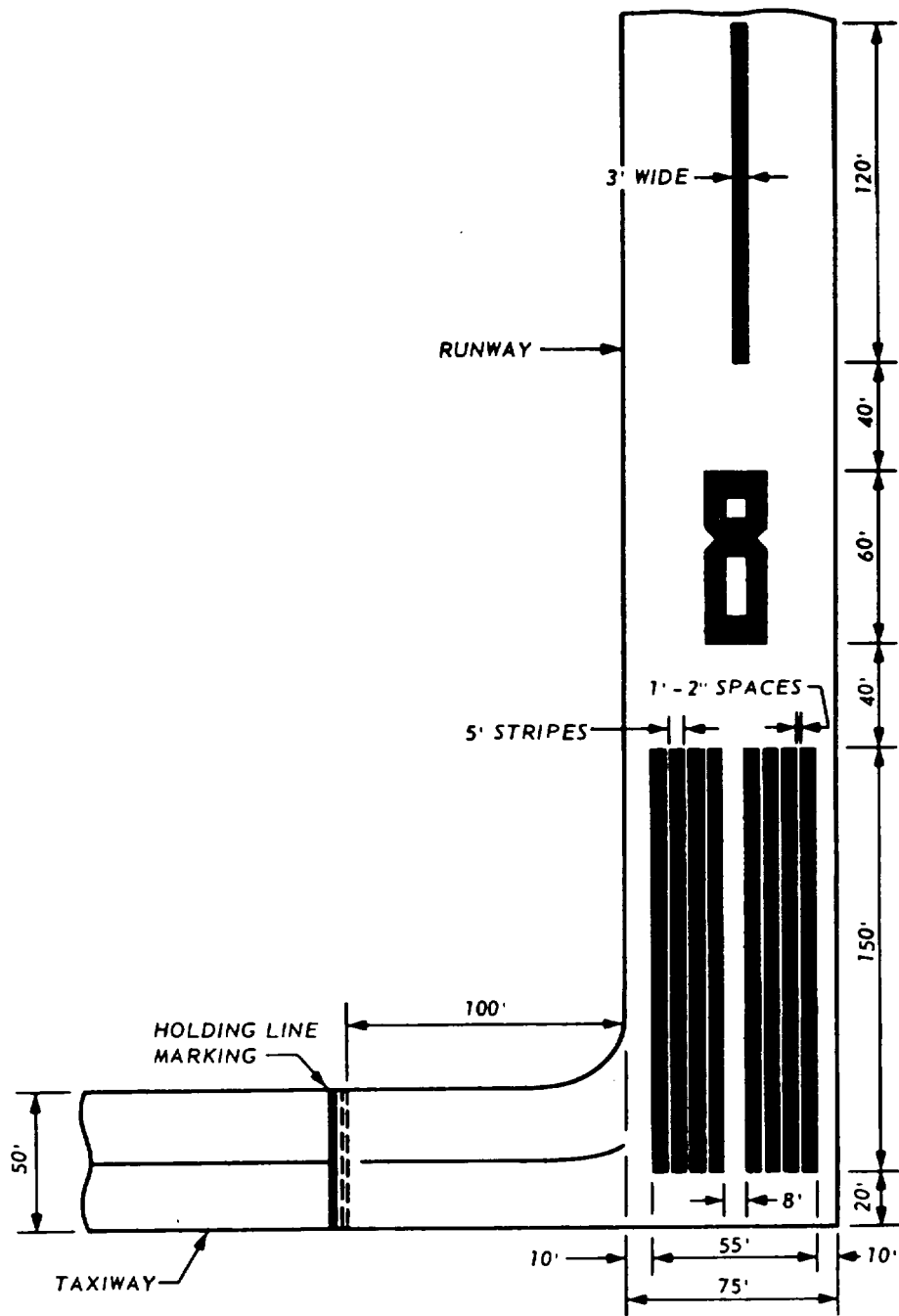
Figure 2-2. Precision instrument runway marking. (Sheet 2 of 2).
