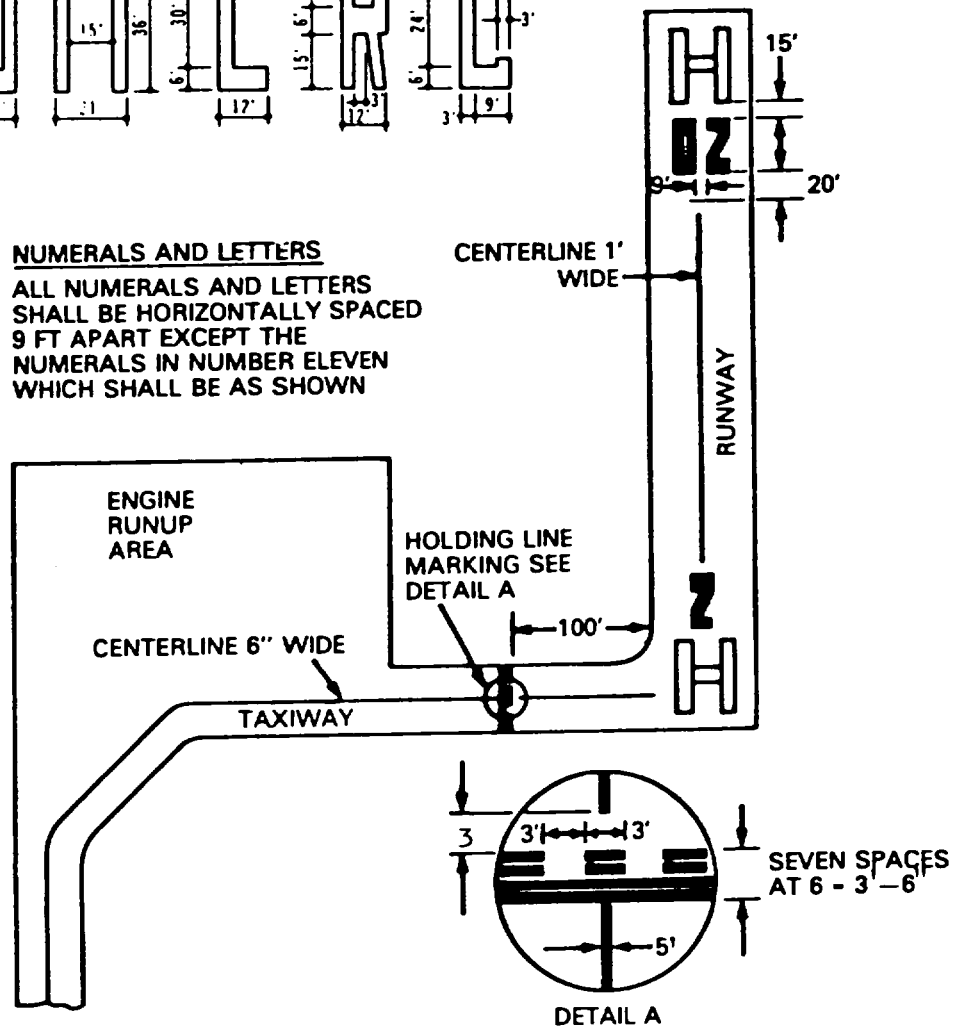
Figure 3-1. Guidelines for marking runways and taxiways at heliports.
