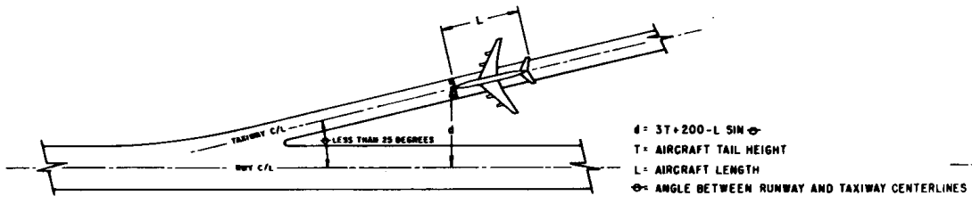
(c) LOCATING HOLDING POSITION LINE FOR TAXIWAY INTERSECTING RUNWAY AT AN ANGLE LESS THAN 25 DEGREES
