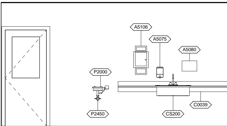
VNEC1 - SOUTH ELEVATION
