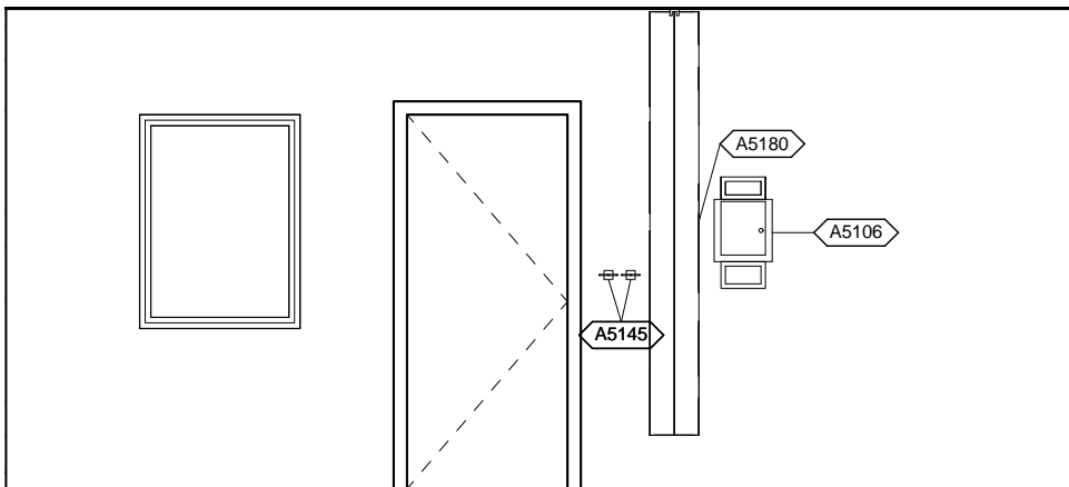
OPIR1 - SOUTH ELEVATION
