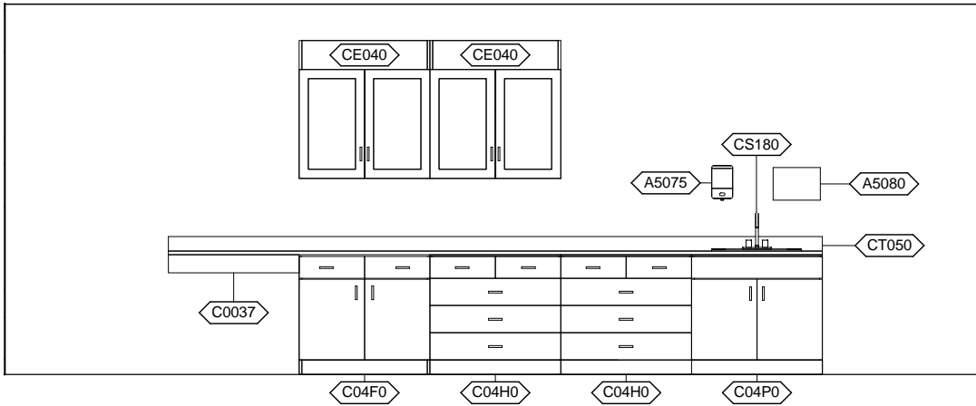
DNSC5 - NORTH ELEVATION
