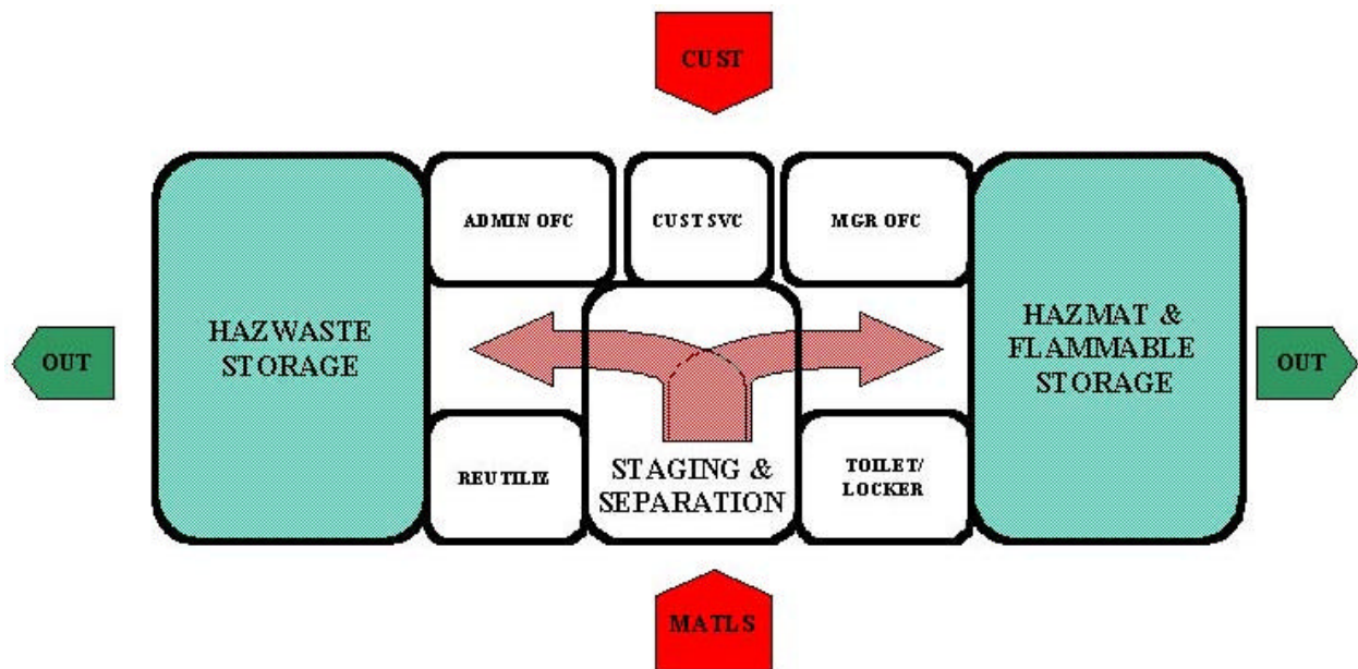
FIGURE B: FUNCTION AREA RELATIONSHIPS
